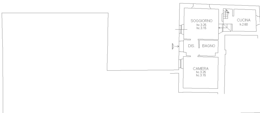
PIANO TERRA
