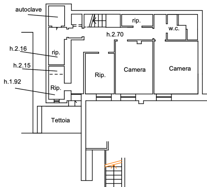
PIANO TERRA
