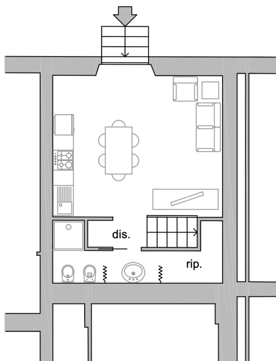
PIANO TERRA
